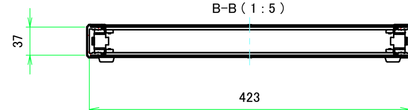
B-B (1:5)
